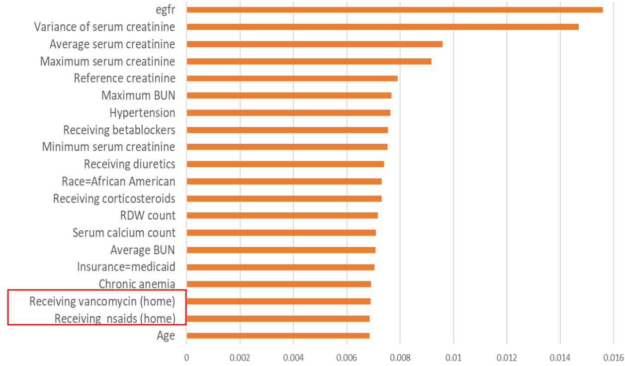
E) Feature importance for model with EHR and home medications
